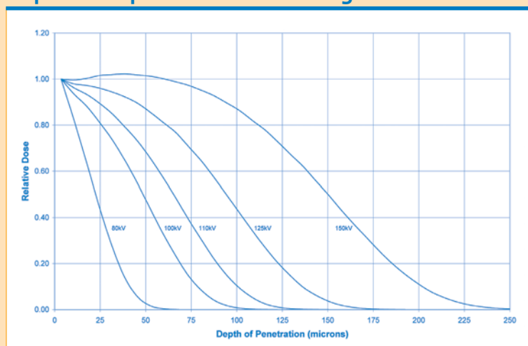
Depth/dose profiles for low-voltage EB
